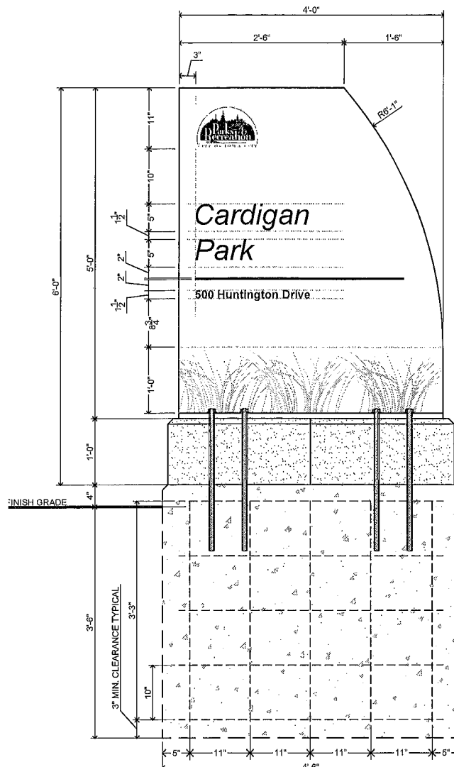
1 N6 SECTION/ELEVATION: PARK IDENTIFICATION SIGN "A" NT.2
