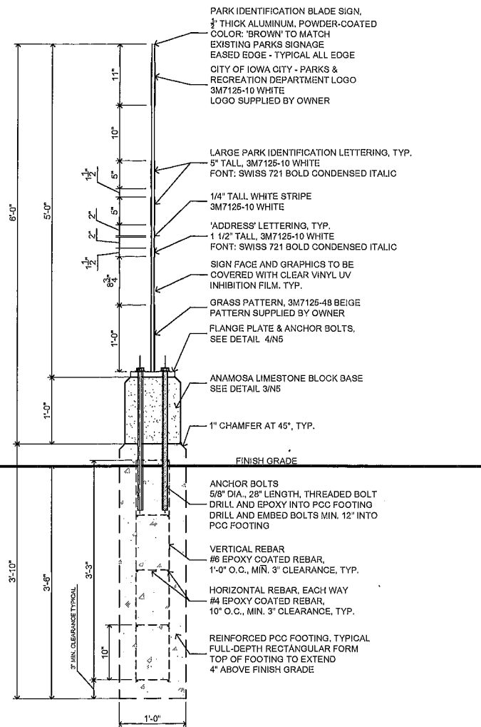
2 N5 SECTION: SIGN "A" NT.2
