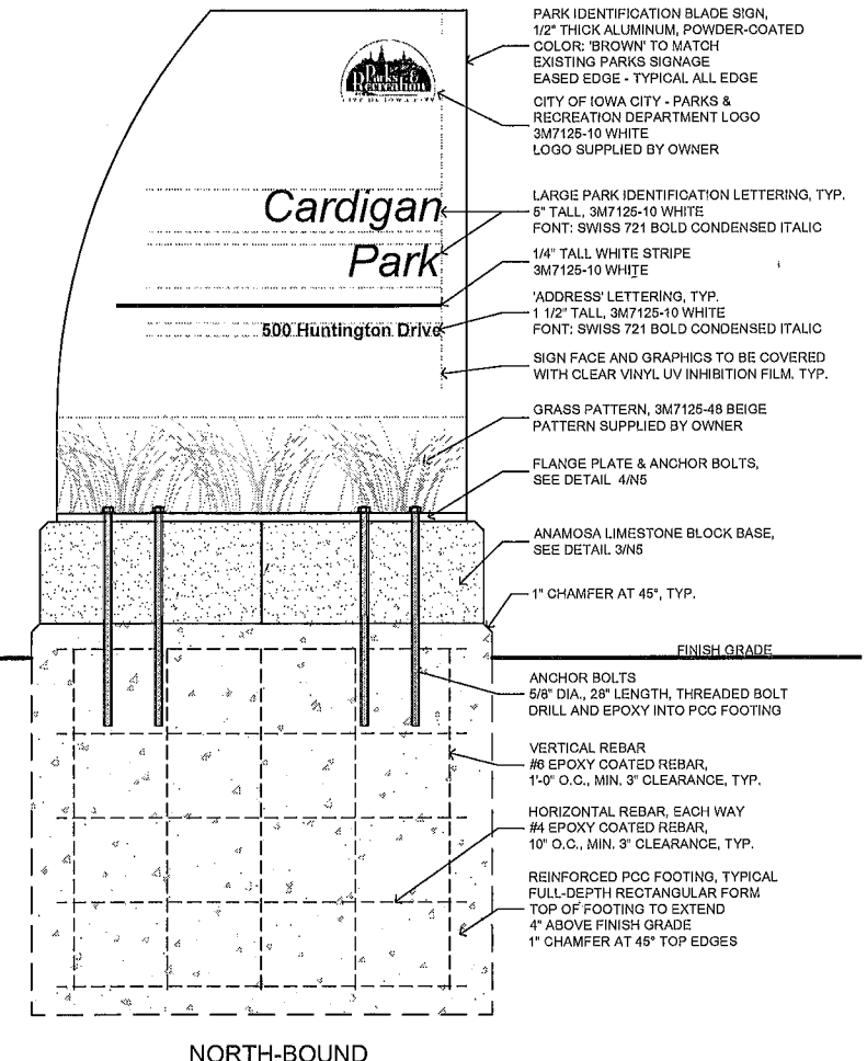
1 N6 SECTION/ELEVATION: PARK IDENTIFICATION SIGN "A" NT.2
